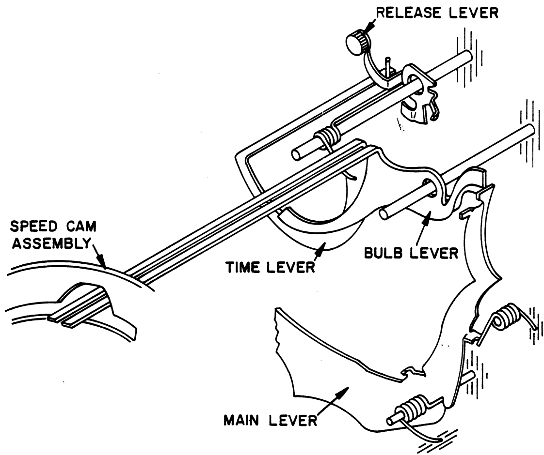
Figure 5. TIME AND BULB LEVER OPERATION
