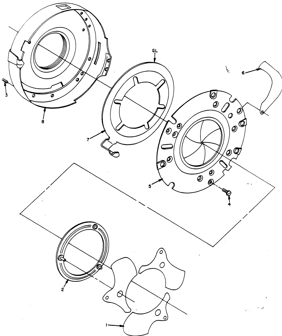
Figure 13. NO. 1 SHUTTER, DISASSEMBLY - STAGE 6
