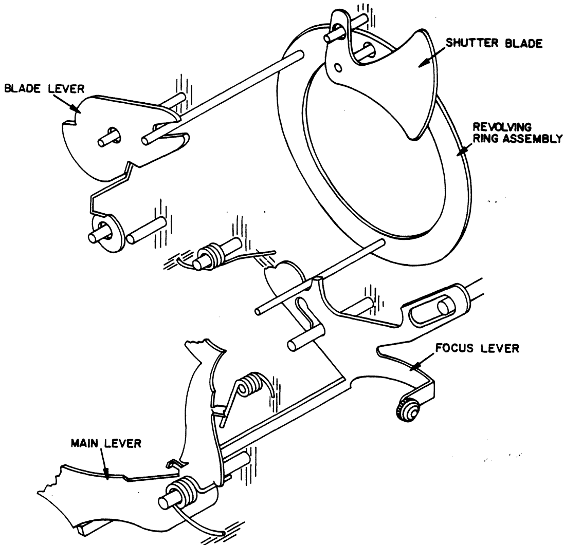
Figure 4. BLADE CLOSING MECHANISM
