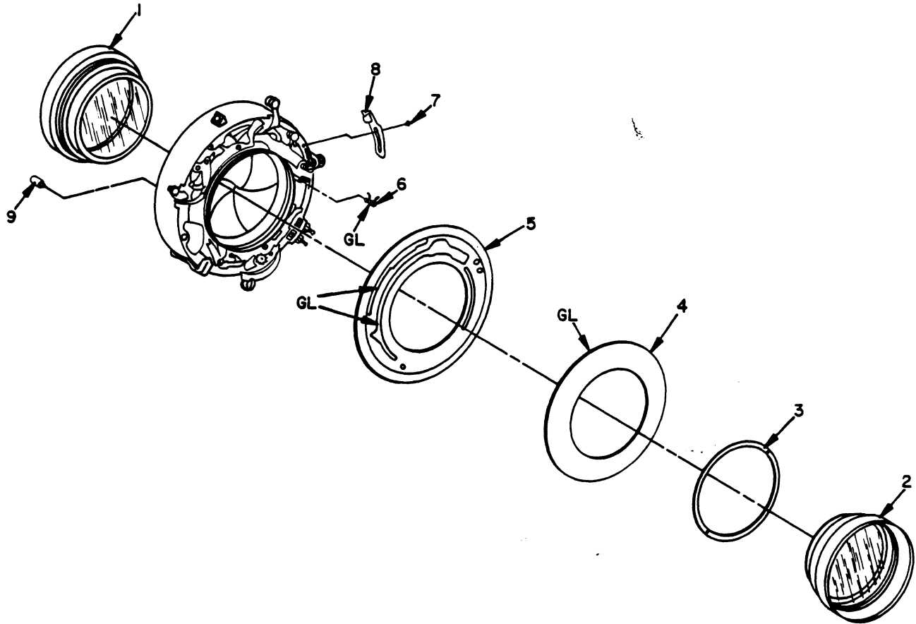
Figure 14. NO. 2 AND 3 SHUTTER, DISASSEMBLY - STAGE 1
