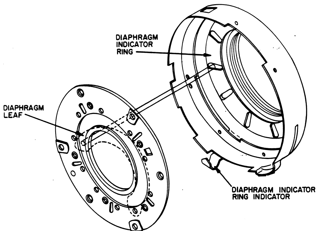
Figure 6. DIAPHRAGM OPERATION
