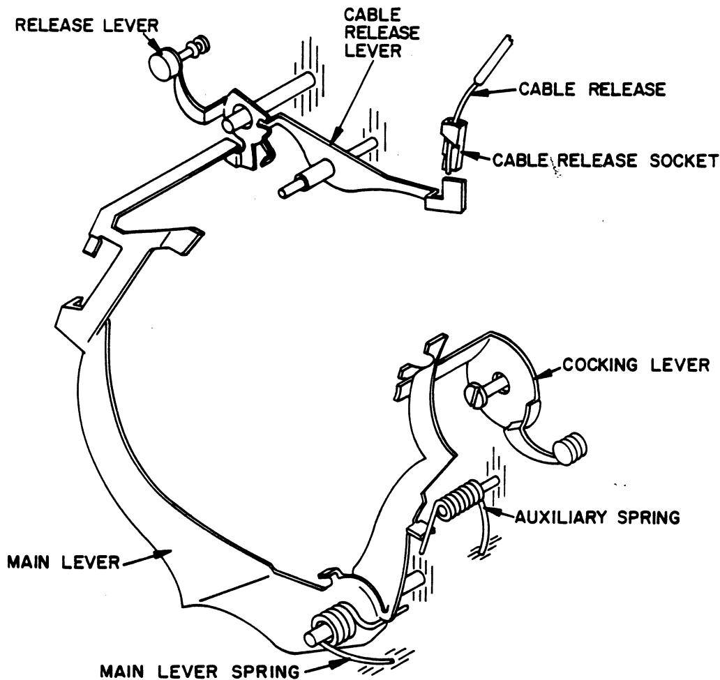
Figure 3. COCKING AND TRIPPING MECHANISM
