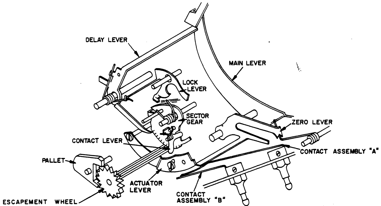
Figure 7. SYNCHRONIZER OPERATION
