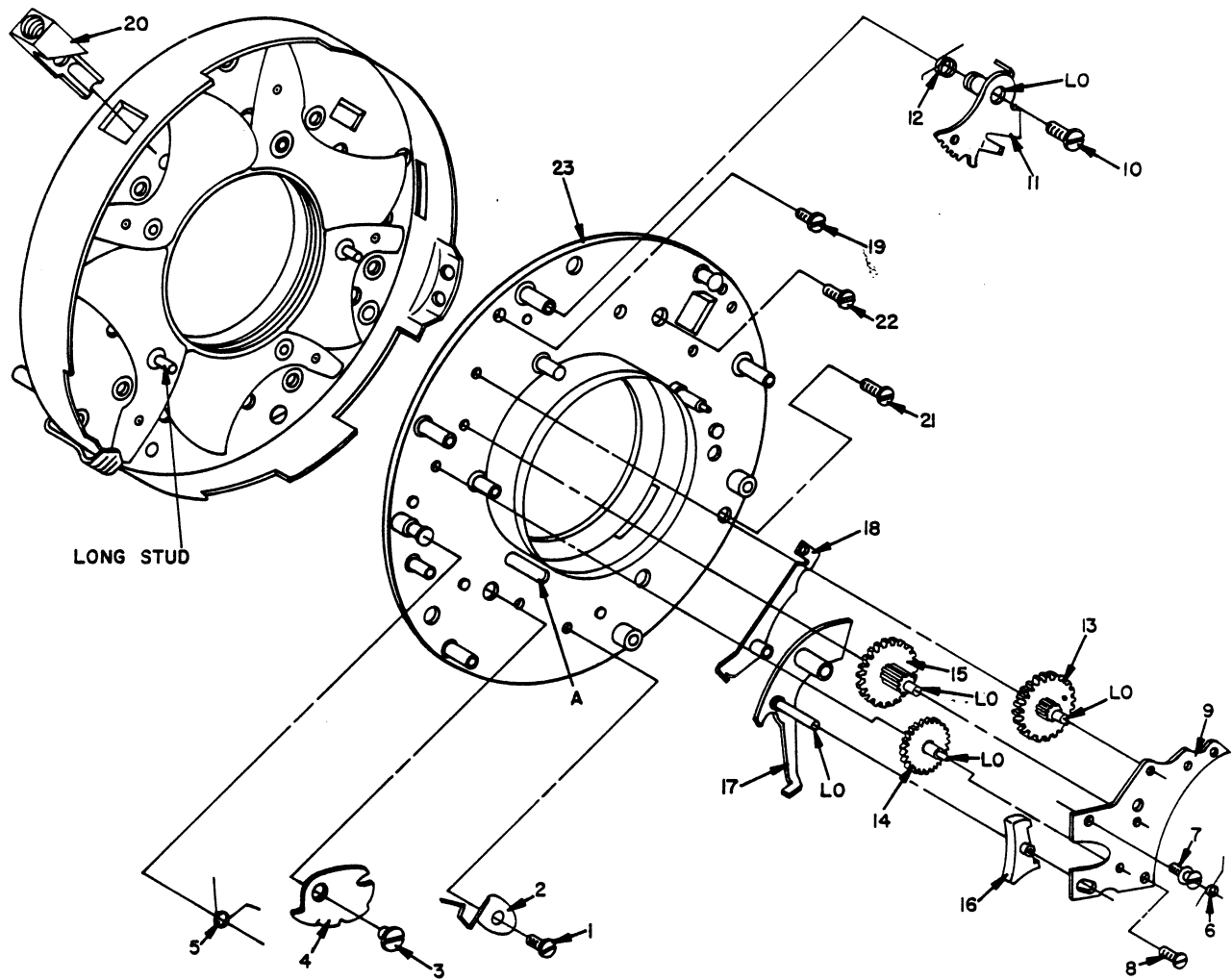
Figure 18. NO. 2 AND 3 SHUTTER, DISASSEMBLY - STAGE 5
