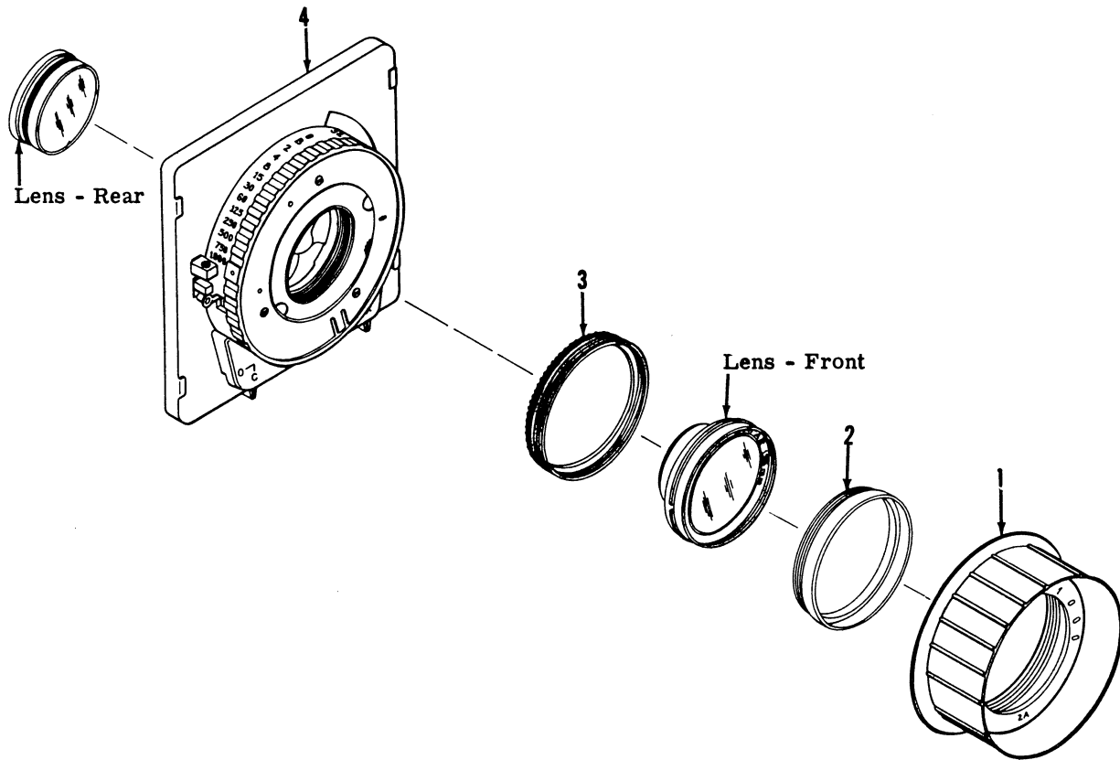
Figure 21. GRAFLEX 1000 SHUTTER
