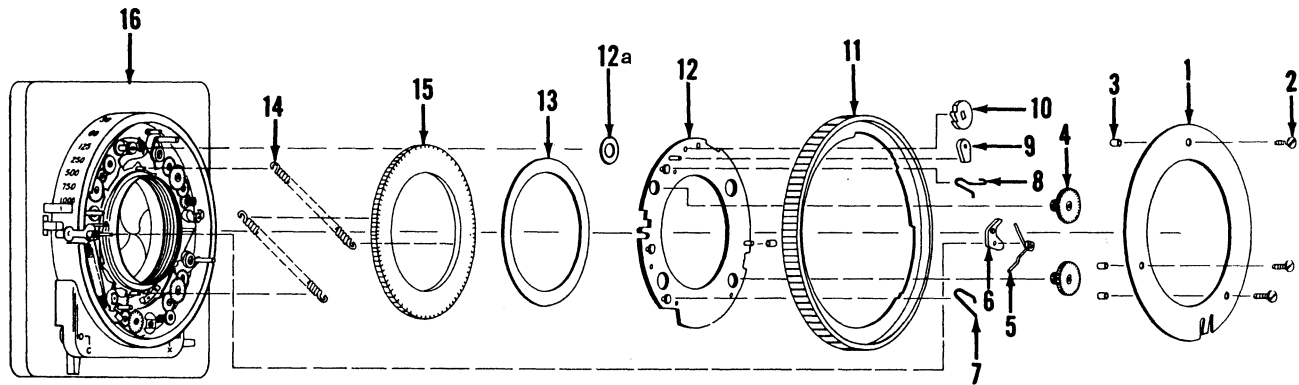
Figure 22. SHUTTER ASSEMBLY - THIRD
