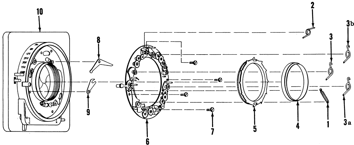
Figure 23. SHUTTER ASSEMBLY - SECOND
