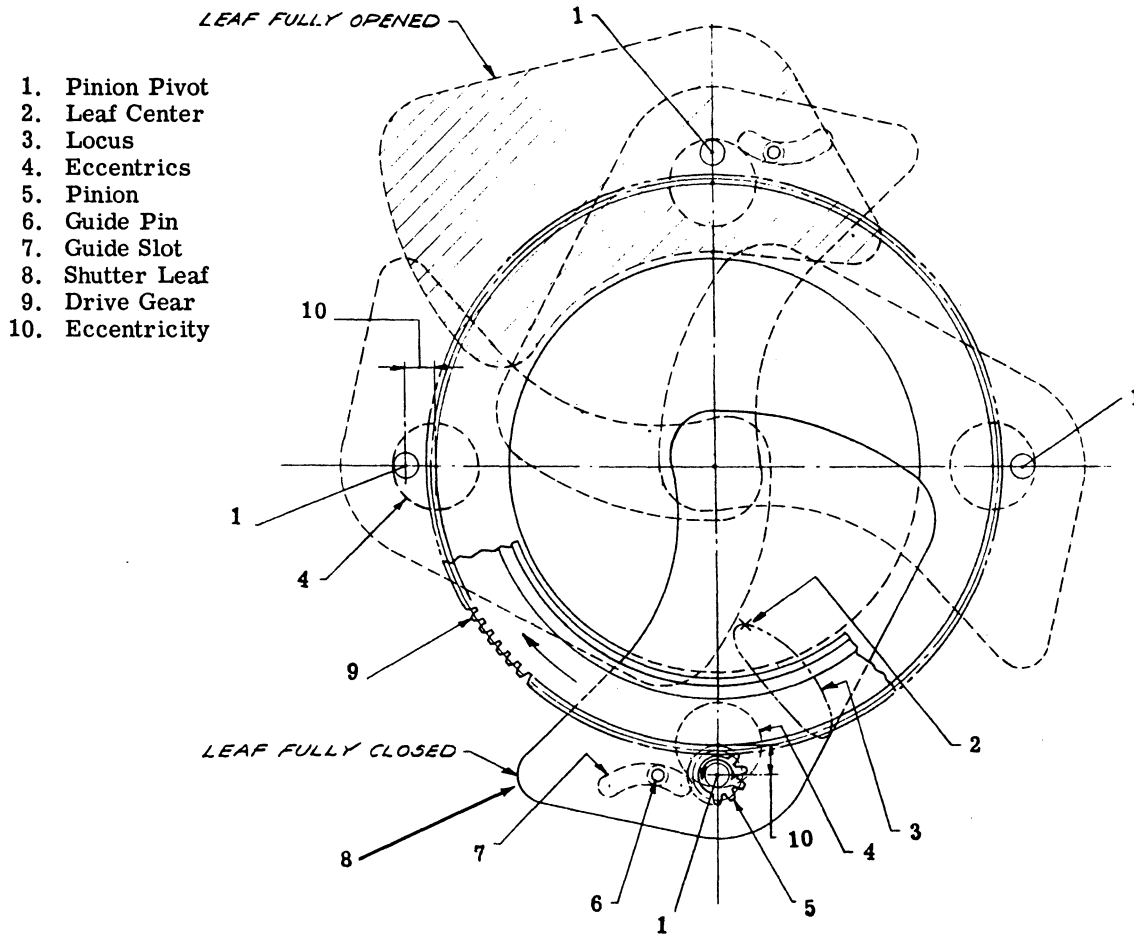
SHUTTER LEAF DRIVE, SCHEMATIC DRAWING
