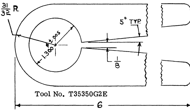
Figure 1. TUBULAR WRENCH (use on front lens element)
